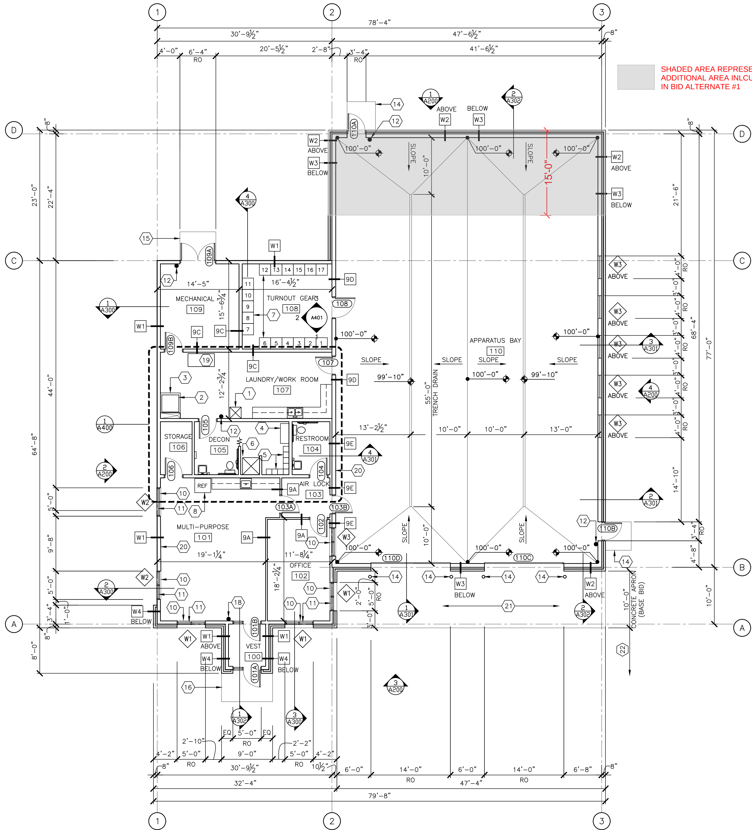
1 FLOOR PLAN - ALTERNATE #1 0 4'-0" 8'-0" 12'-0" FINISHED FLOOR ELEVATION (FFE) = 100'-0" = 1031'.00
